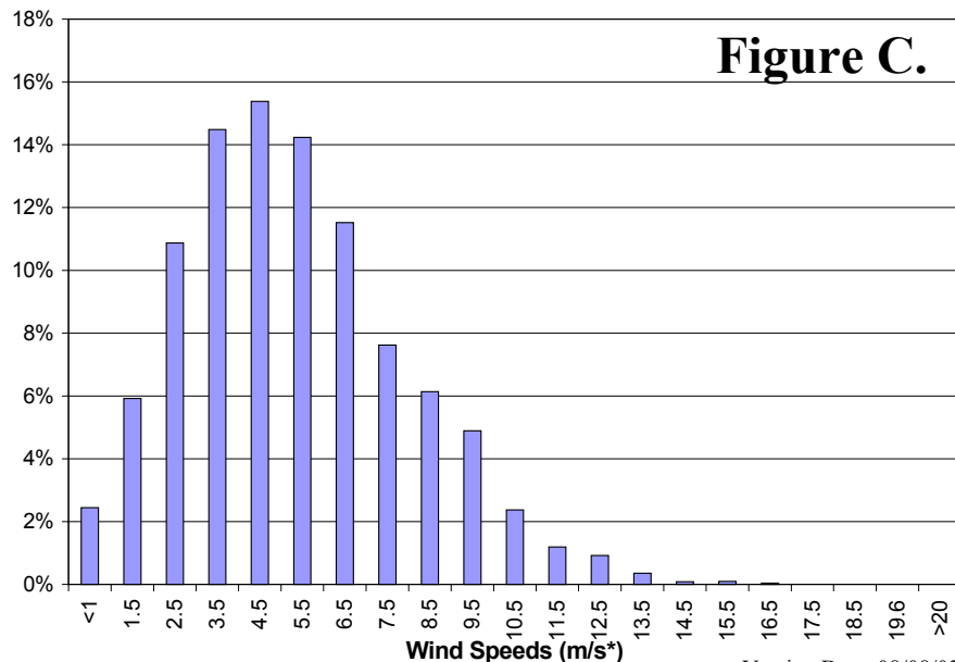
Frequency Distribution of Wind Speeds at 50 meters
